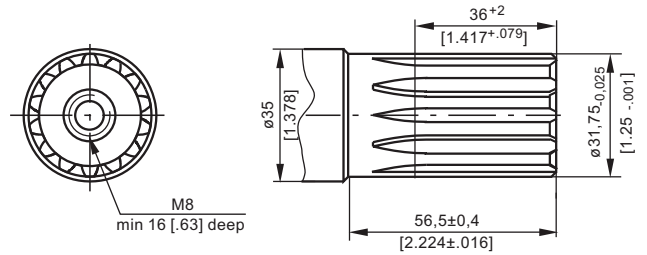
SH - \phi 1\frac{1}{4} " splined 14T, DP12/24 ANS B92.1-1970 Max. Torque 95 daNm [8400 lb-in]
