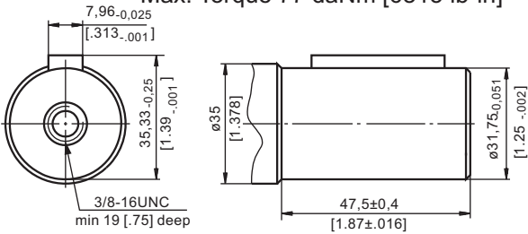
CO - \phi 1\frac{1}{4} " straight, Parallel key \frac{5}{16} "x \frac{5}{16} "x 1\frac{1}{4} " BS46 Max. Torque 77 daNm [6815 lb-in]
