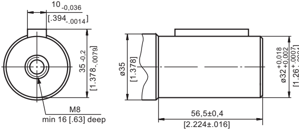
C - \phi 32 straight, Parallel key A10x8x45 DIN 6885 Max. Torque 77 daNm [6815 lb-in]
